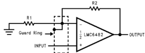
Non-Inverting Amplifier
