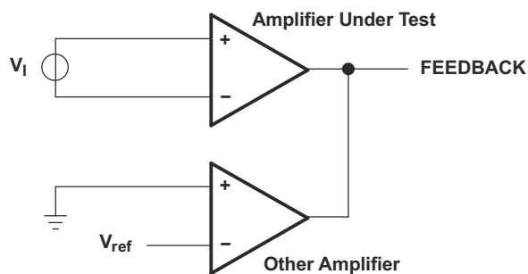
Figure 8-2. Amplifier Characteristics
