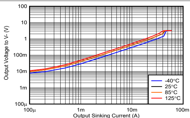
Figure 6-4. Output Voltage vs. Sinking Current, 3.3V
