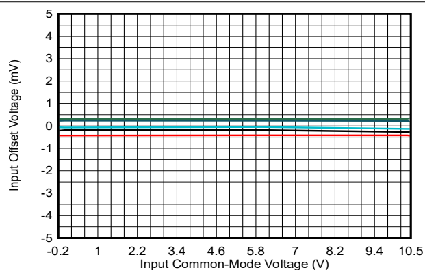
Figure 6-2. Offset Voltage vs. Common-Mode, 12V
